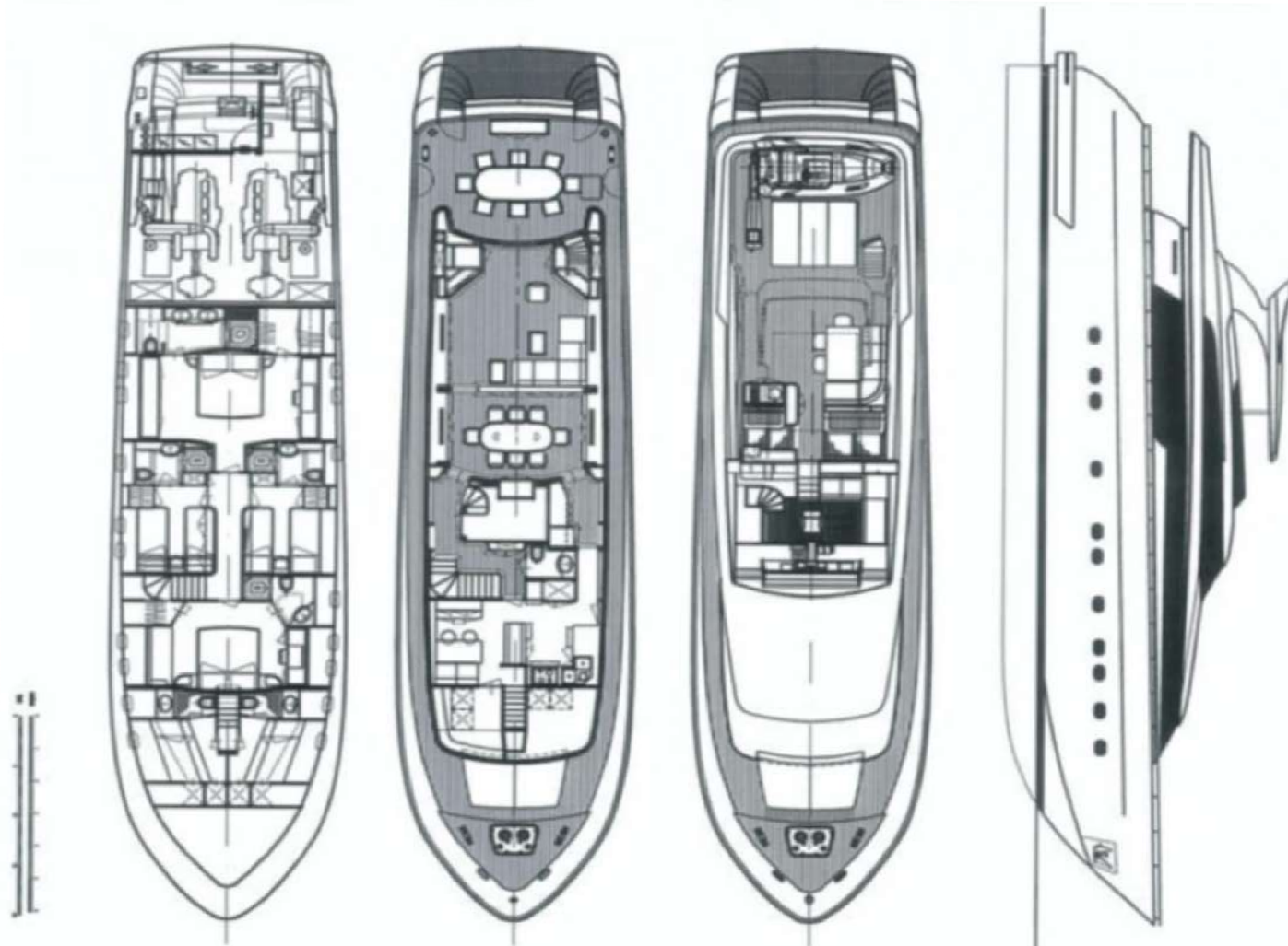
Sanlorenzo SL 88Standard layout
